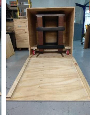
Step 2: Place the lid on the corner of the pallet with the supports prepared for it, and lower the link with the ramp.
